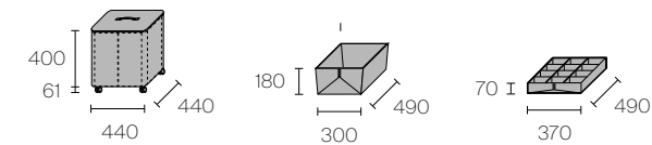
Synthetic leather cabinet on wheels, box and tray
