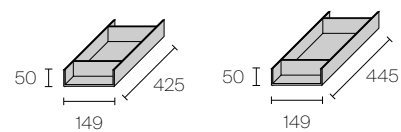
Veneered organizer
