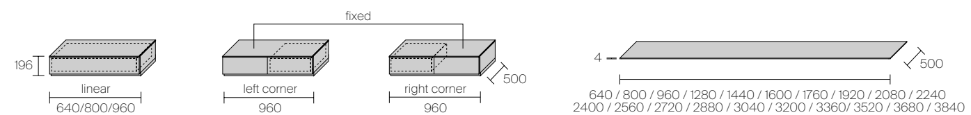
Linear floor unit with drawer
