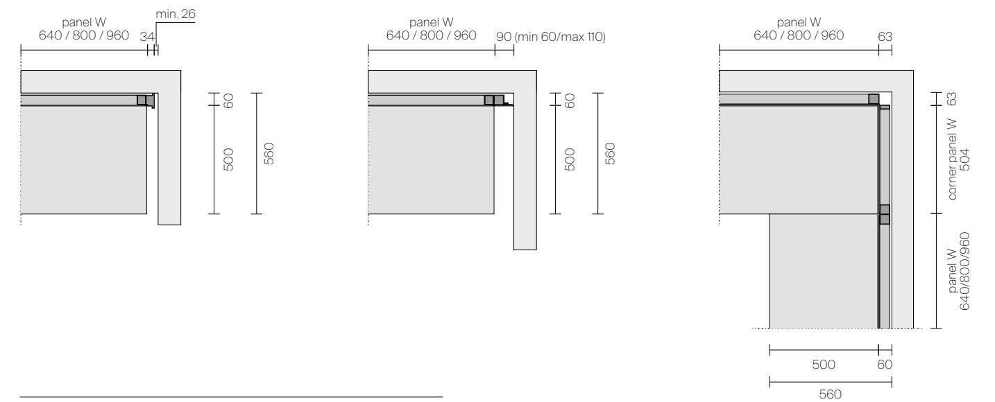
Floor base
